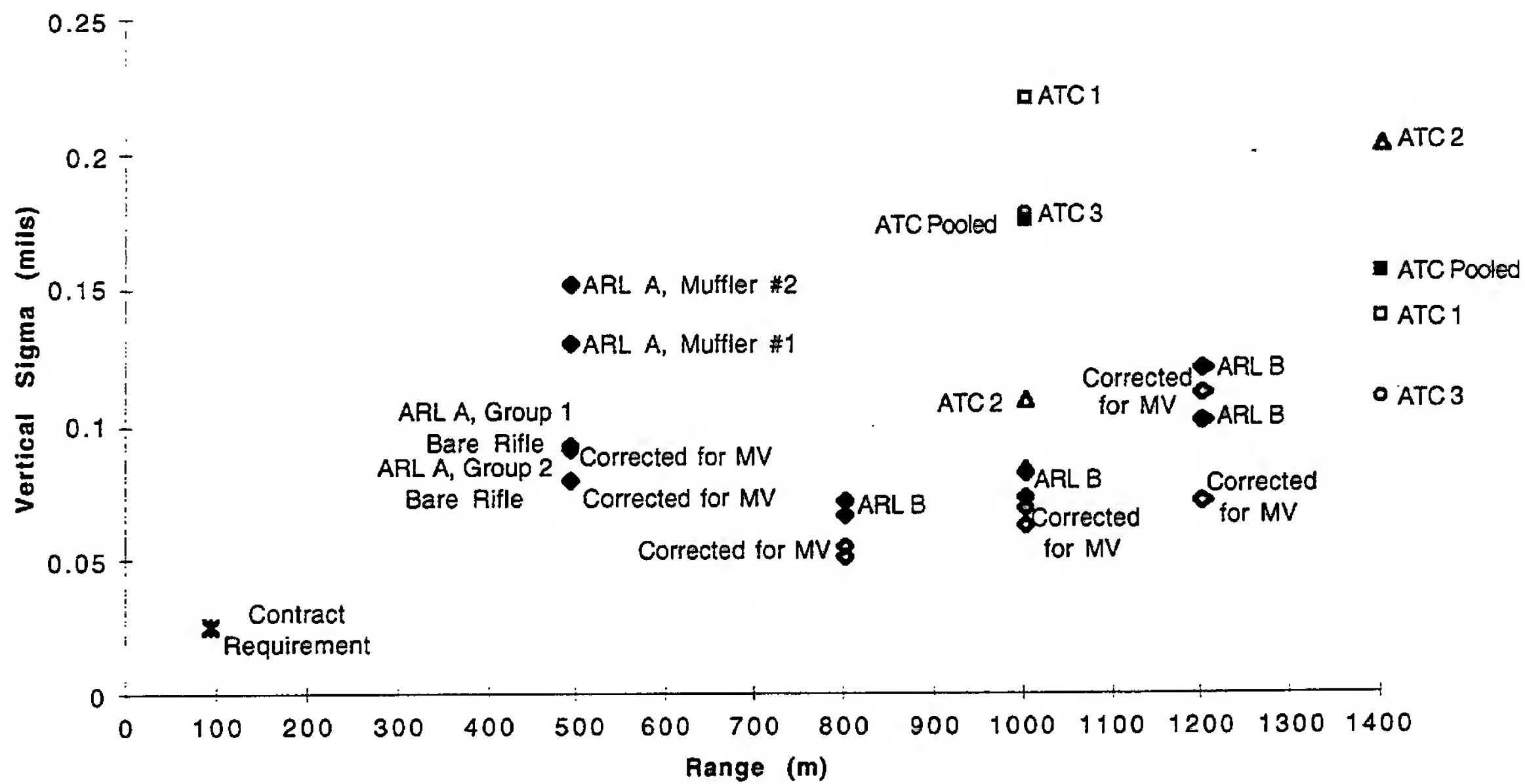
Figure A-4. Vertical Dispersion Data, .338-.416.
